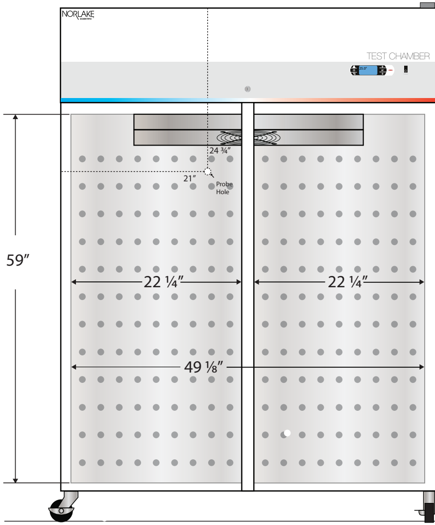
Front View
